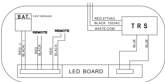
Exit RC Wiring Diagram:
