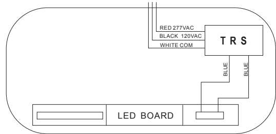
AC Only Wiring Diagram:
