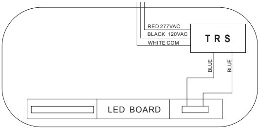
AC Only Wiring Diagram:
