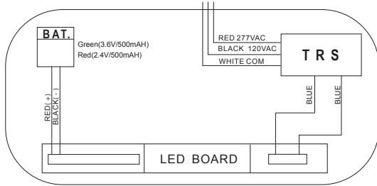
Exit Battery Wiring Diagram:
