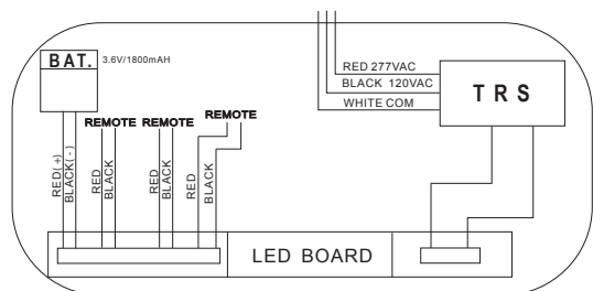
Exit Battery RC Self-Diagnostic
