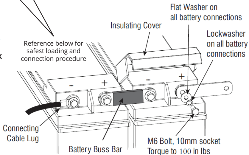
INVERTER BATTERY CABLE CONNECTION TERMINAL BLOCK 2 battery strings (parallel connections)
