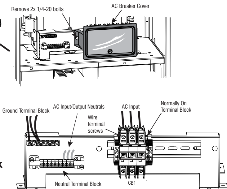
Standard Output Terminal Block Illustration
