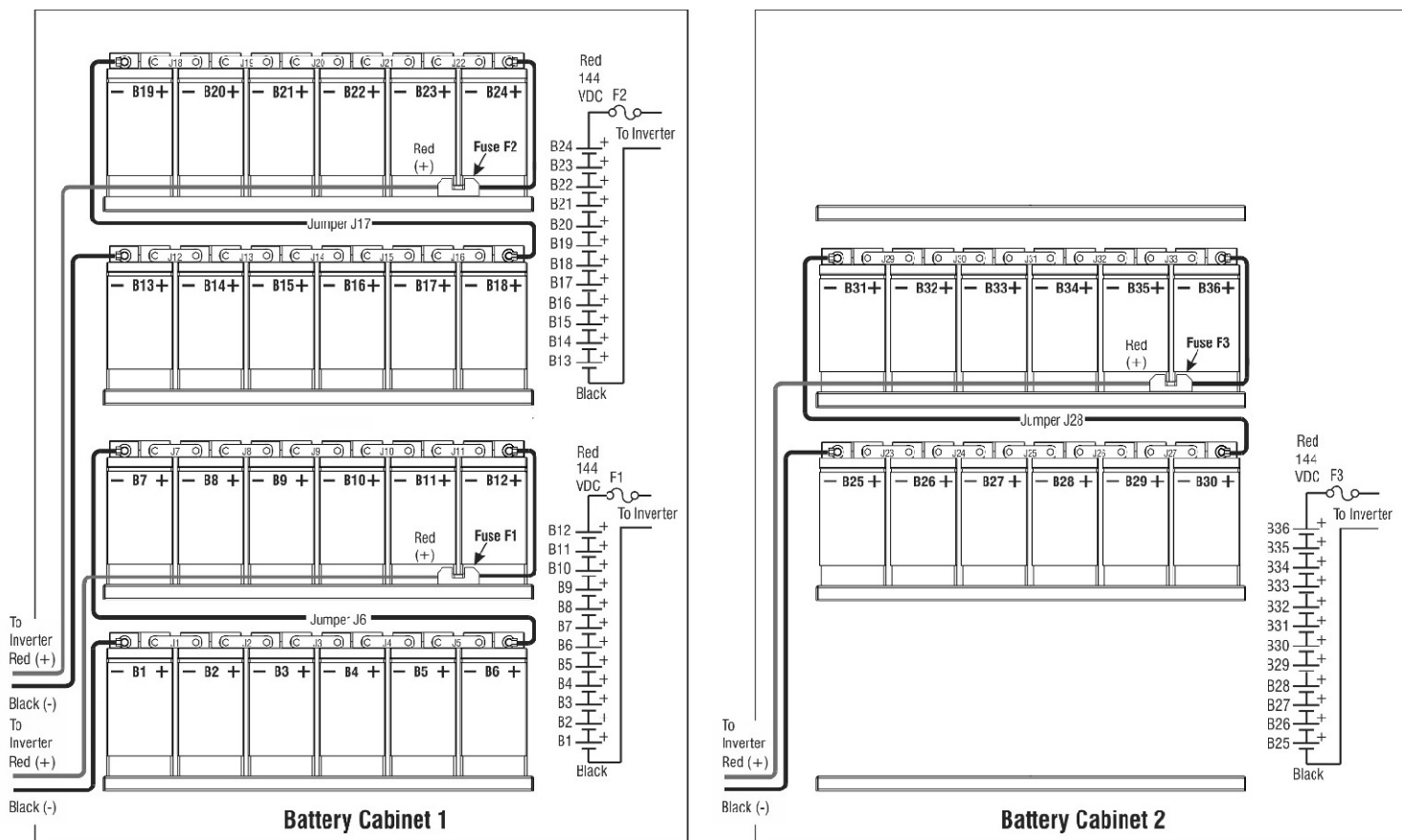
Three String Battery Connection - 144 VDC Systems
