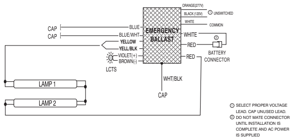
B. Two (2) Lamp Without AC Ballast
