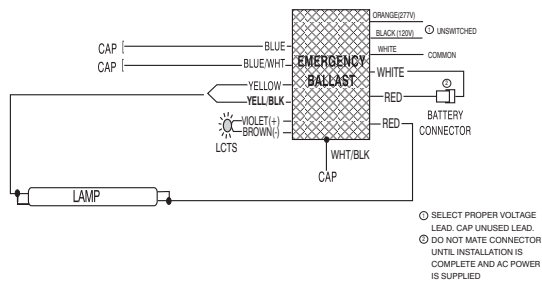
A. One (1) Lamp Without AC Ballast
