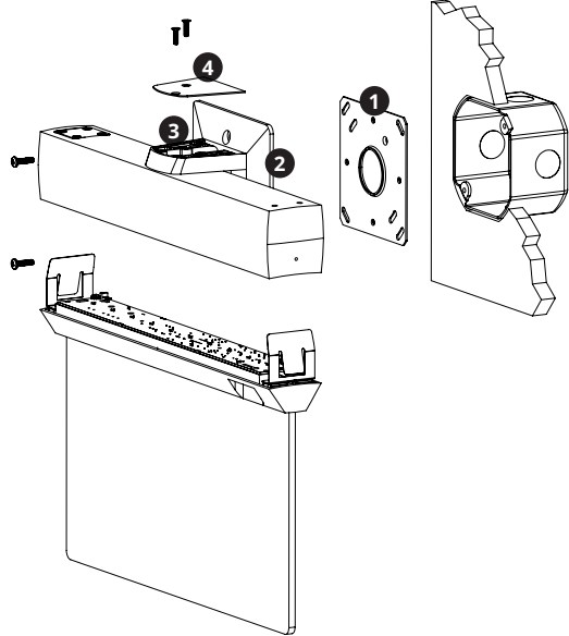
FIGURE 10: Surface Back
