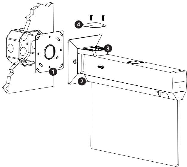
FIGURE 8: Surface End
