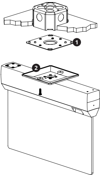
FIGURE 9: Surface Ceiling
